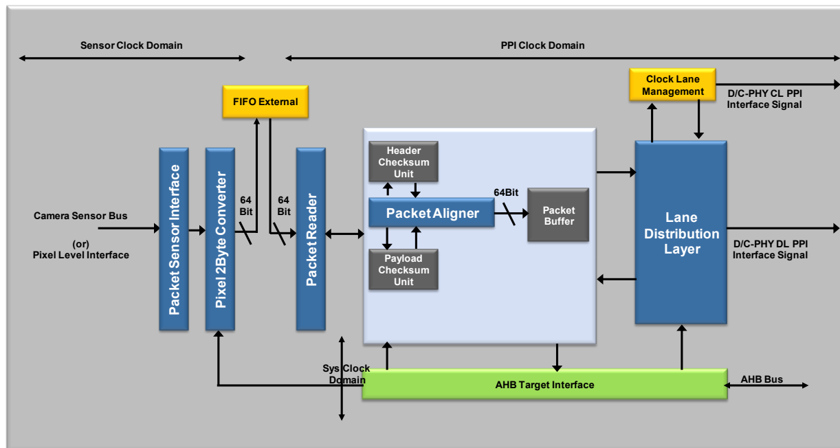
Figure 1 Combo Transmitter Functional Block Diagram
